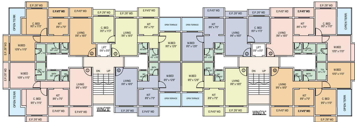
1ST,3RD & 5TH FLOOR PLAN
